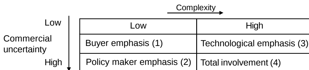
Figure. 7.3: Fisher's Model
